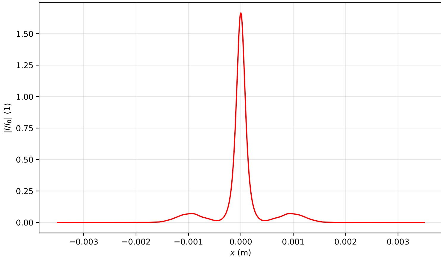
Intensity profile I(x, y = 0, z = 2.388)/I_0 , P_{in}=8.0P_{cr} , artificial time
